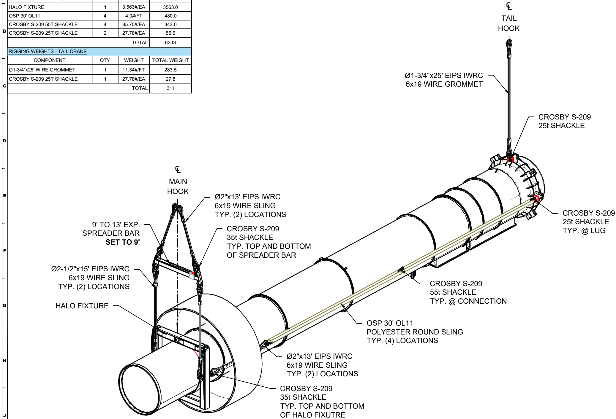
ISOMETRIC VIEW
