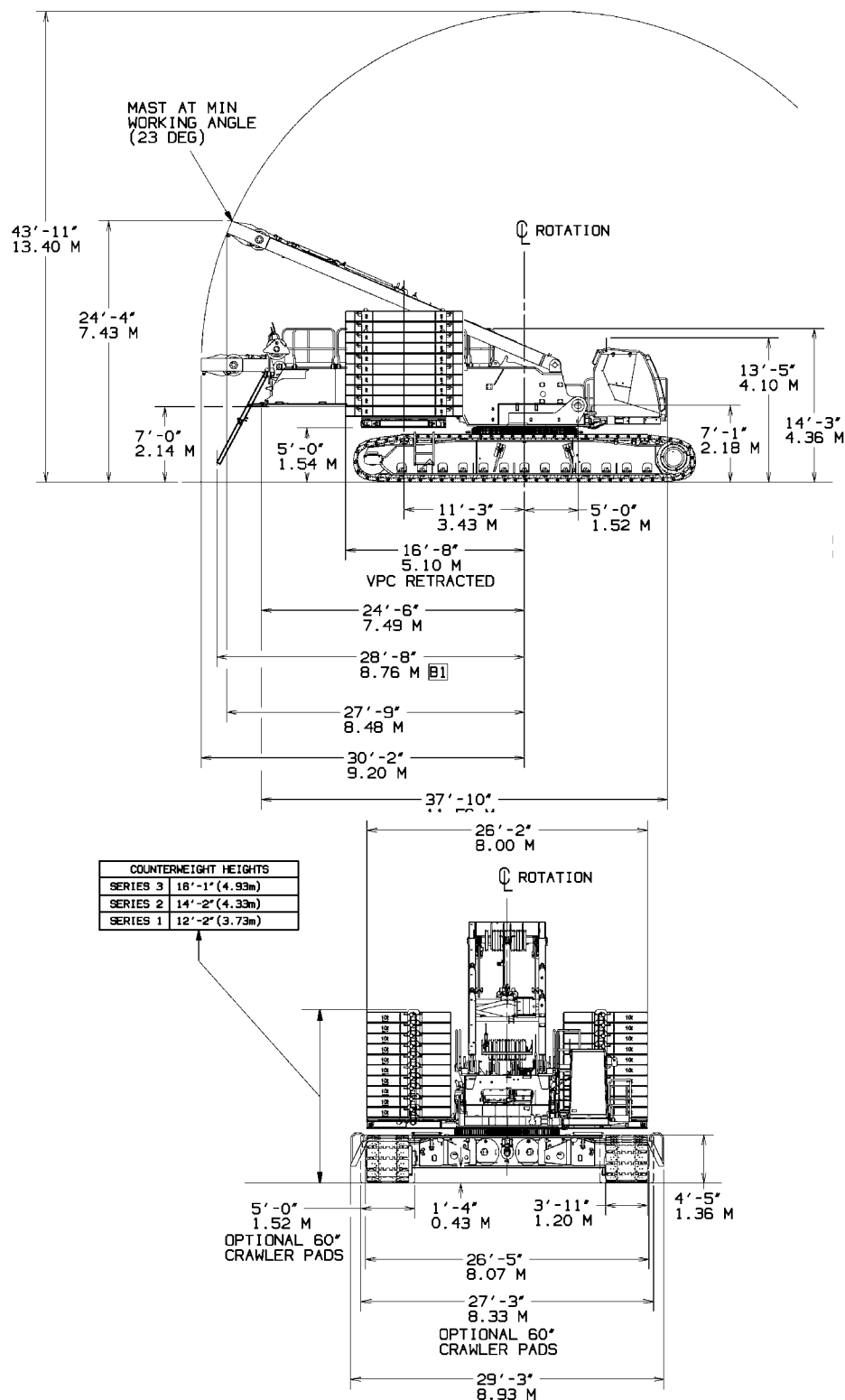
Manitowoc MLC300
