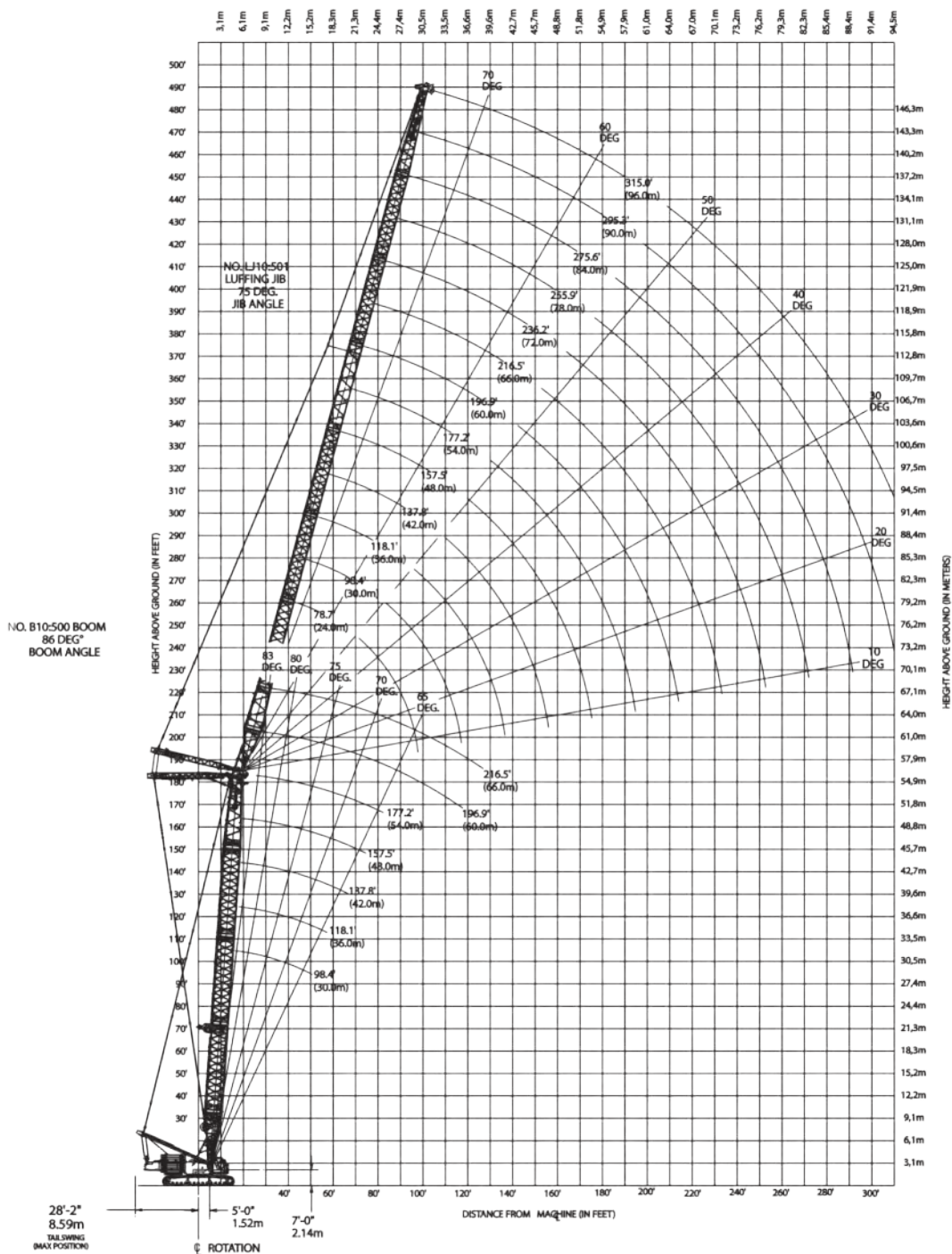
LJ10:501 luffing jib on B10:500 boom
